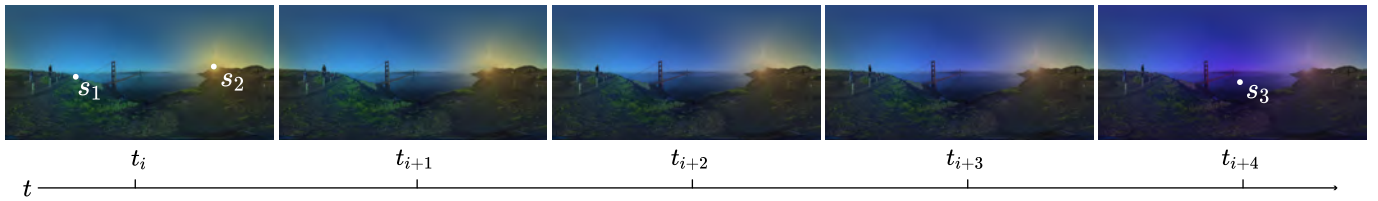
Figure 4. Visualization of parameter interpolation. Spatial keyframes s_1 (cyan) and s_2 (yellow) at time t_i and s_3 (purple) at time t_{i+4} , interpolate both spatially and temporally using radial basis functions. Note this does not represent the in-headset viewing experience because any single pixel will have different parameters applied to it depending on the users’ view.
